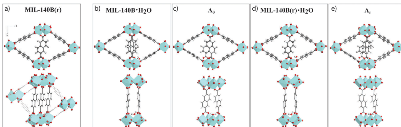
Fig. 4 Crystal structure of MIL-140B(r) , formed by rotating 50% of the ndc linkers which lie along the a -axis, around the b -axis by 180°. Structures of MIL-140B contain one \text{H}_2\text{O} molecule per unit cell viewed along the c -axis. Models called MIL-140B-H 2 O and MIL-140B(r)-H 2 O contain an uncoordinated water molecule, while A 0 and A r are defective models and are built with a \text{H}_2\text{O} molecule coordinates directly to a Zr-center. The latter displaces the linker which becomes monodentate on one its carboxylate end. Zr atoms are depicted as light blue polyhedra, O is red, C is gray and H is white.
