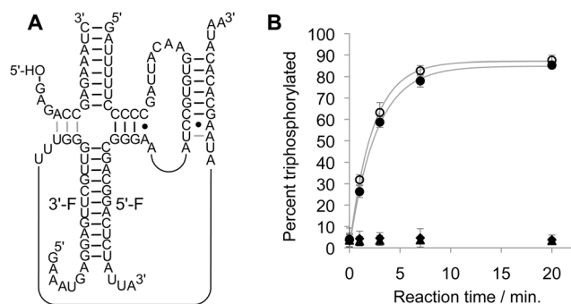
Fig. 2 Fragmentation of the ribozyme in the loop of the P5 stem. (A) Secondary structure of the fragmented ribozyme, labeling its 5'-fragment (5'-F) and the 3'-fragment (3'-F). (B) Reaction kinetics of the full-length, unfragmented ribozyme (empty circles), the 5'-fragment alone (filled triangle), the 3'-fragment alone (filled diamonds), and the combination of 5'-fragment and 3'-fragment (filled circles). Error bars are standard deviations from three experiments; if error bars are not visible they are smaller than the symbols.
