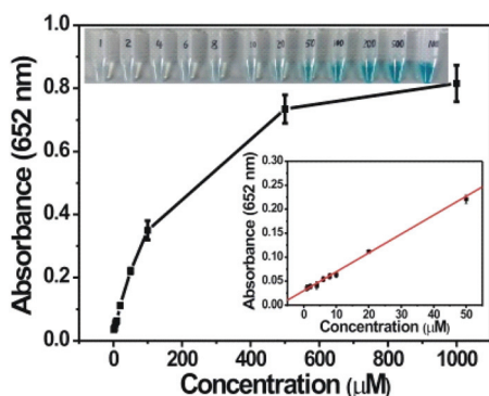
Fig. 5 Dependence of the absorbance at 652 nm on the concentration of H 2 O 2 from 1 \mu M to 1 mM. The upper and lower insets show the corresponding photographs of different solutions and linear calibration plot, respectively.
