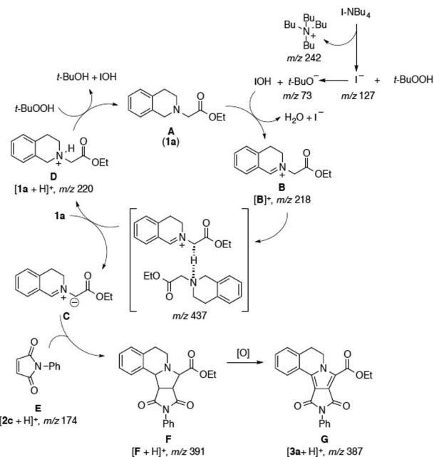
Scheme 1 Proposed mechanism.
