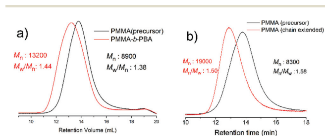
Fig. 2 Comparison of the GPC traces of precursor PMMA with (a) PMMA- b -PBA and (b) chain extended PMMA.
