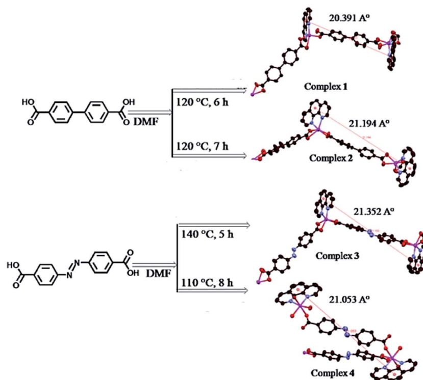
Scheme 14 CPs obtained by the reaction of metal [\text{Zn(II)}] , [\text{Cd(II)}] , phen separately with biphenyl-4,4'-dicarboxylic acid and 4,4'-azodibenzoic acid. [Reprinted with permission from ref. 170. Copyright 2012, American Chemical Society.]
