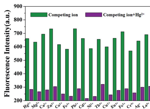
Fig. 2 Fluorescence of PP5 ([RU] = 4 \times 10^{-5} M) at 470 nm with addition of 10.0 equiv. of \text{Hg}^{2+} in the presence of 10.0 equiv. of other cations in DMSO/ \text{H}_2\text{O} (1 : 1, v/v).
