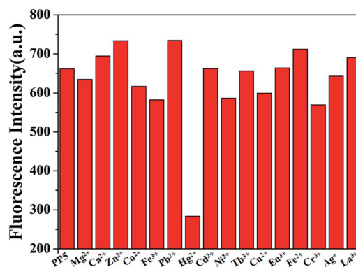
Fig. 1 Fluorescence spectra responses for PP5 ( [RU] = 4 \times 10^{-5} M) and each of the various cations ( 4 \times 10^{-4} M) in DMSO/H 2 O (1 : 1, v/v).
