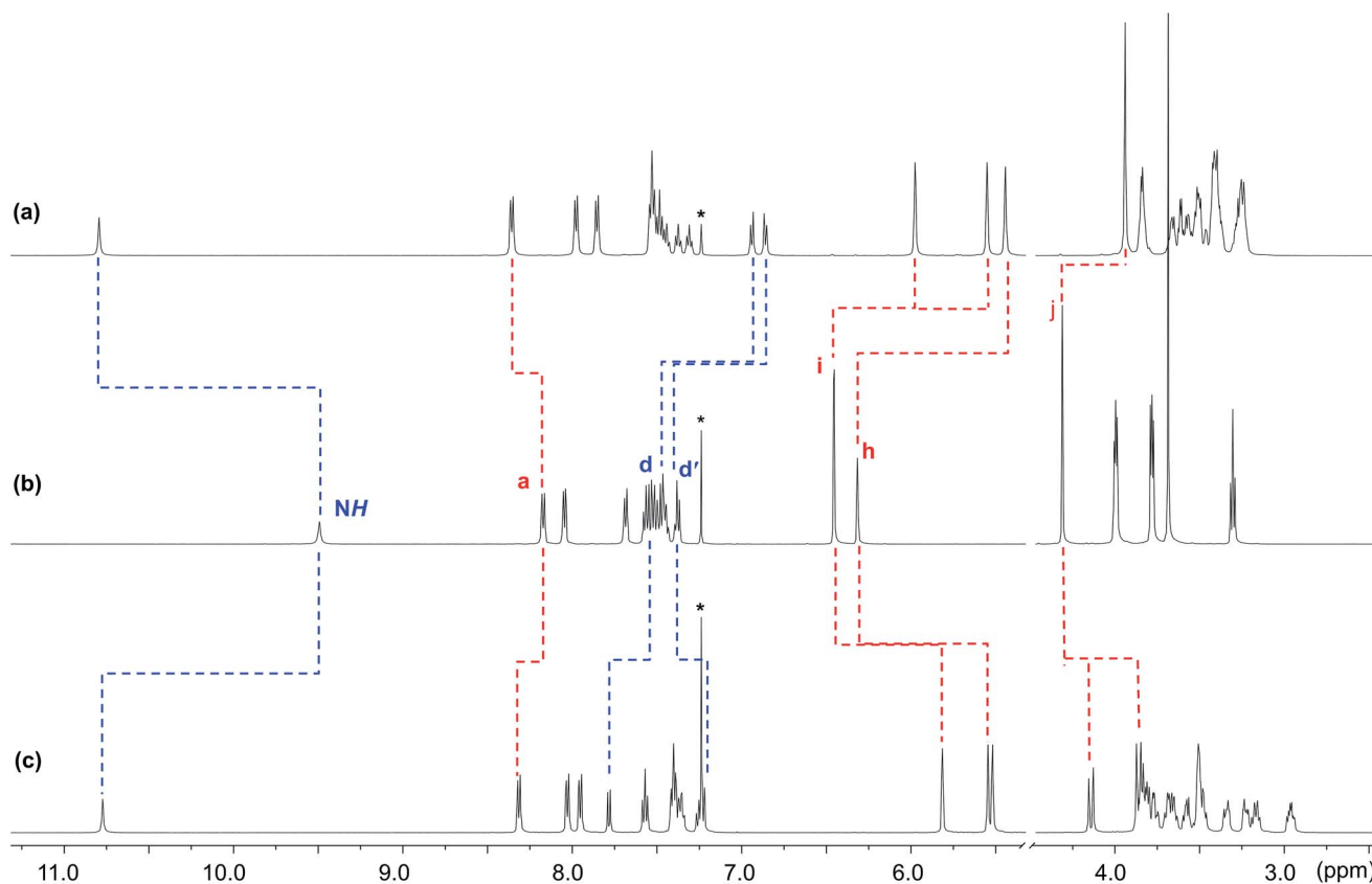
Fig. 2 Comparison of the partial ^1\text{H} NMR spectra (500 MHz, \text{CDCl}_3 ) of (a) suit[1]ane 6a , (b) an equimolar solution of 1 and 7 and (c) suit[1]ane 6b (* = \text{CHCl}_2 ). Labelling scheme is shown in Scheme 2 for 1 and 7 .
