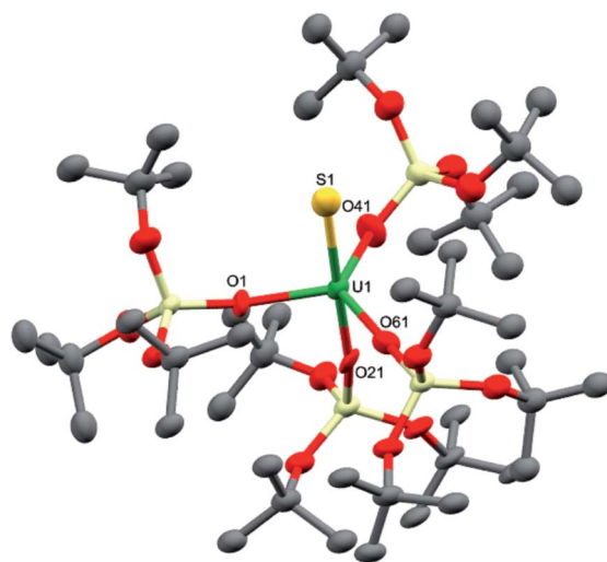
Fig. 5 Molecular structure of the anionic fragment of one of the crystallographically independent pairs of [K(2.2.2-cryptand)][U\{OSi(OtBu)_3\}_4] in crystals of 8·1.5tol shown with 50% probability thermal ellipsoids. [K(2.2.2-cryptand)]^+ , hydrogen atoms and lattice solvent molecules have been omitted for clarity.
