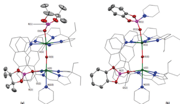
Fig. 1 Solid-state structures of 2-2toluene (a) and 3-THF (b). Displacement ellipsoids are drawn with 50% probability, and carbon atoms of L^A and U-coordinated solvent molecules drawn wireframe. For clarity, hydrogen atoms, lattice solvent, and lower-fractional occupancy disorder components of the OBpin ligand (B(1)), and L^A ethyl groups of 2-2toluene are omitted.
