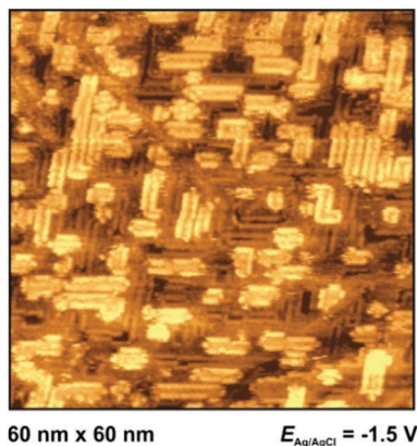
Fig. 10 Interfacial structure of PMPiF 6 N on Au(100).
