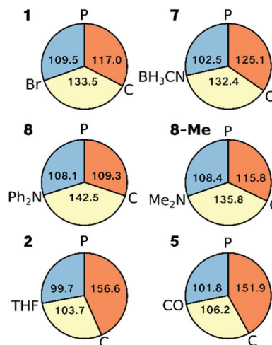
Fig. 9 Pie diagrams representing the angles around the Ni ion in the crystal structures for 1 , 2 , 5 , 7 , 8 and the geometry optimised structure of 8-Me ; orange: \angle\text{P-Ni-C} , yellow: \angle\text{C-Ni-L} , blue: \angle\text{L-Ni-P} , where L stands for the respective ligand.
