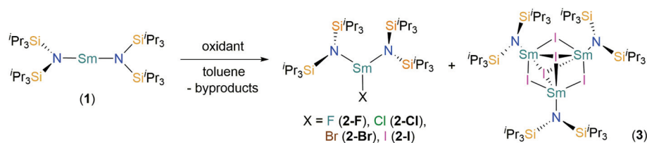
Scheme 1 Synthesis of [\text{Sm}(\text{N}^{\text{III}})_2(\text{X})] ( \text{X} = \text{F} , 2-F ; \text{Cl} , 2-Cl ; \text{Br} , 2-Br ; \text{I} , 2-I ) and [\{\text{Sm}(\text{N}^{\text{III}})\}_3(\mu_2\text{-I})_3(\mu_3\text{-I})_2] ( 3 ) by the treatment of [\text{Sm}(\text{N}^{\text{II}})_2] ( 1 ) with various oxidants; 2-F : +\text{[Fe(Cp)}_2\text{][PF}_6\text{]} , -\text{[Fe(Cp)}_2\text{]} , and \text{PF}_5 ; 2-Cl , 2-Br : +^t\text{BuX} , -\text{CH}_3\text{CH}(\text{CH}_3)\text{CH}_3 , and -\text{CH}_2=\text{C}(\text{CH}_3)\text{CH}_3 ; 2-I , 3 : +0.5 \text{ I}_2 and -\text{unidentified by-products} .
