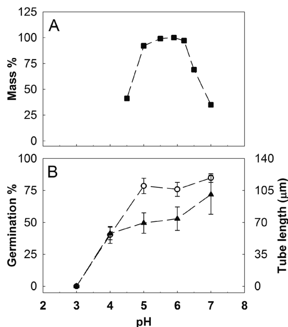
Fig. 7 Percentage of pollen tube mass development in N. tabacum [redrawn from Tupí and Řihová (1984)] (A) and germination percentage (—○—) and pollen tube length (—▲—) of Corylus avellana (B) as a function of pH. Values in B are means \pm 1 st. dev ( n = 450 in A; n = 90 in B).
