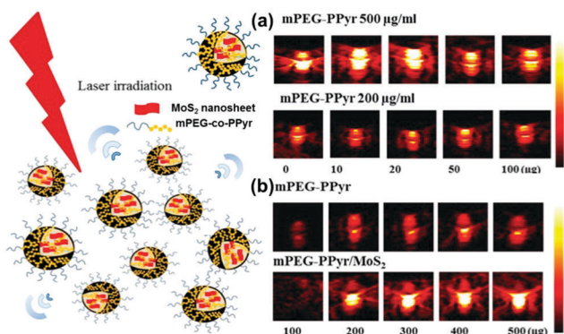
Fig. 7 Photoacoustic activity of mPEG-co-PPyr nanoparticles and mPEG-co-PPyr/MoS 2 nanocomposites. (a) PA signal of mPEG-co-PPyr/MoS 2 NCs with varied MoS 2 concentrations (0–100 μg), and (b) PA signal of mPEG-co-PPyr/MoS 2 NCs at constant MoS 2 concentration (20 μg) and with a varied concentration of mPEG-co-PPyr (100–500 μg). All mPEG-co-PPyr/MoS 2 NCs complexed with MoS 2 showed significantly enhanced photoacoustic activity. The average energy density of the laser irradiation was 14.48 mJ cm -2 in each experiment of (a) and (b). The inner and outer diameters of the used tygon tubes were ID 0.05 in, OD 0.09 in, and ID 0.04 in, OD 0.07 in, respectively, for experiments (a) and (b). Reprinted with permission from ref. 71. Copyright 2016 American Chemical Society.
