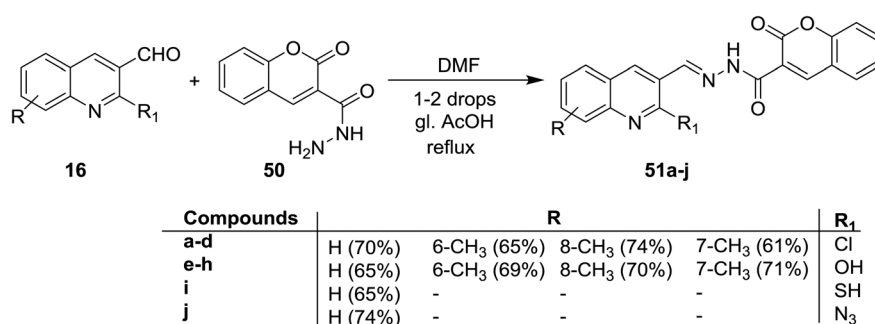
Scheme 10 Condensation of 16 with carbonylhydrazide.
