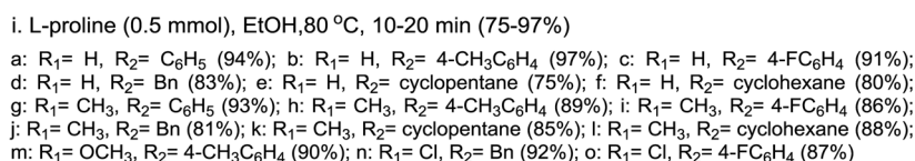
Scheme 31 Synthesis of 4 H -thio-pyrano[2,3- b ]quinolines.
