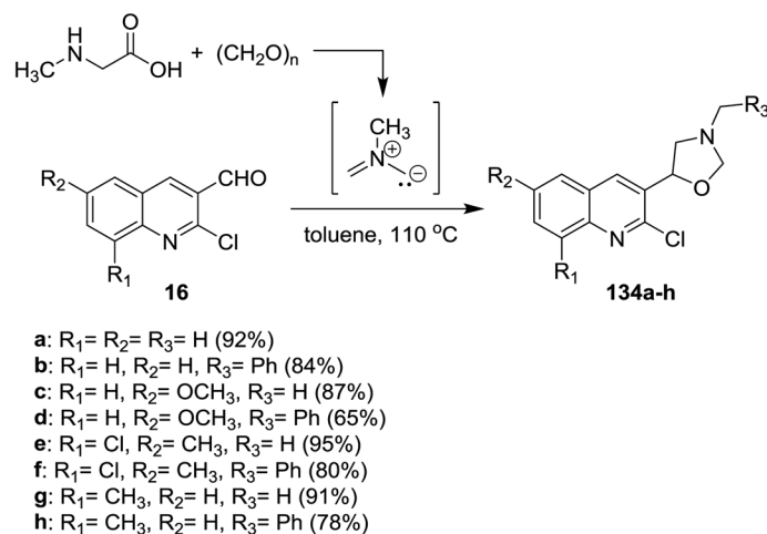
Scheme 45 Synthesis of 2-chloroquinoliny-oxazolidines.
