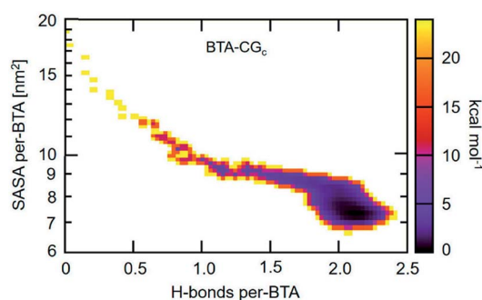
Fig. 19 2D self-assembly free energy landscape of BTA-CG model as a function of average number of H-bonds per BTA and average SASA per BTA. This figure has been reproduced from ref. 96 with permission from the American Chemical Society.
