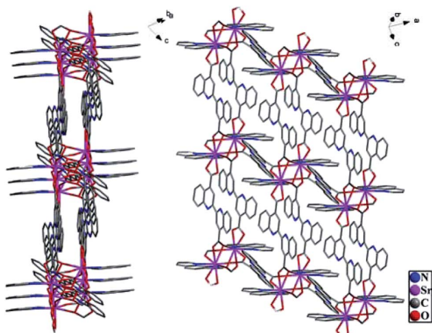
Fig. 1 Illustration of the \text{MOCPh}_2\text{Sr}_2(\text{bqdc})_3(\text{phen})_2 . All of the H atoms are omitted for clarity.
