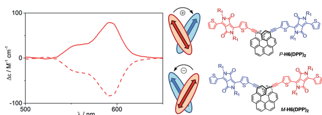
Fig. 6 Relation between the helical arrangement of the DPP units around the P - or M -helicenic core and the respective positive or negative exciton coupling signature.
