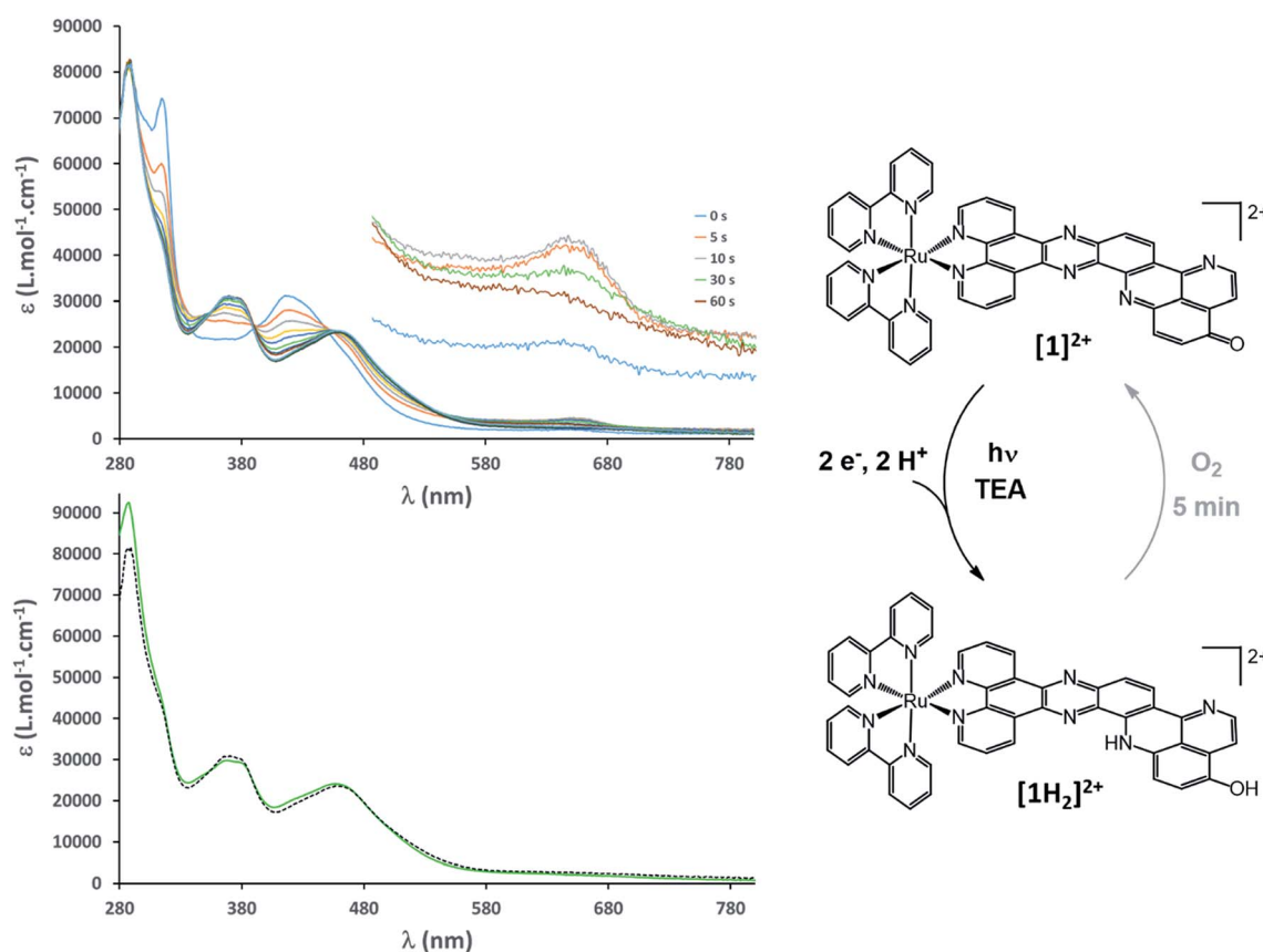
Fig. 3 Top: UV/vis monitoring of a continuous photolysis experiment ( \lambda_{\text{exc}} = 450 \text{ nm} ; 15 \mu\text{M} in \text{CH}_3\text{CN} in the presence of 0.15 \text{ M TEA} (inset: zoom-in of the 600\text{--}700 \text{ nm} area where the formation of [\mathbf{1}]^+ is observed). Bottom: comparison of the photolysis experiment ( t = 5 \text{ min} ; dotted line) with [\mathbf{1H}_2]^{2+} (green line). Right: summary scheme of the reversible light-driven charge accumulation process.
