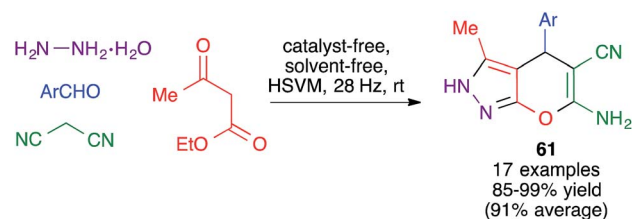
Scheme 42 Mechanochemical synthesis of pyrano[2,3-c]pyrazoles.
