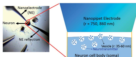
Fig. 3 Measurement of vesicle density. The measured vesicle density is \sim 25 \pm 2 vesicles per \mu m ^2 . The vesicle radius ( r ) is reported in ref. 30.
