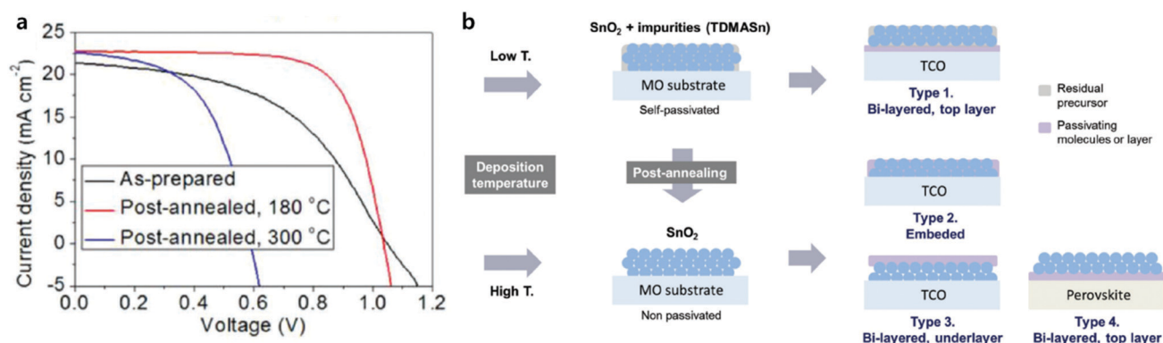
Fig. 6 (a) J–V curve change according to the post-annealing of ALD SnO 2 films. (b) Self- and post-passivation of the ALD SnO 2 films. Low-temperature deposition results in incomplete conversion of the precursor, which remains on the SnO 2 film as a self-passivating layer. The schematic shows that the surface passivation of SnO 2 films can be controlled by post-annealing. Four different methods of post-passivation are proposed. Reproduced with permission. 55 Copyright 2018, The Royal Society of Chemistry.
