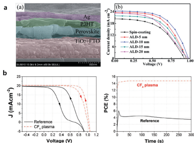
Fig. 4 (a) Cross-sectional SEM image of a perovskite solar cell with FTO/ALD TiO 2 /perovskite/P3HT/Ag layers and J–V curves of solar cells based on conventional TiO 2 and ALD TiO 2 layers (5, 10, 15 and 20 nm). Reproduced with permission. 49 Copyright 2015, The Royal Society of Chemistry. (b) J–V curves of the perovskite solar cells with ALD TiO 2 as the ETL (solid black line) and CF 4 plasma-treated ALD (dash red line); and maximum power point tracking (MPPT) for the two devices. Reproduced with permission. 52 Copyright 2018, Wiley-VCH.
