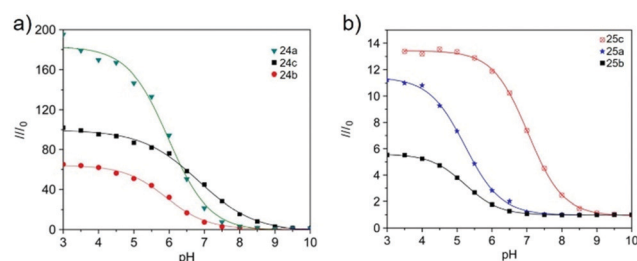
Fig. 36 (a) Fluorescence intensity (at 517 \text{ nm} ) ratios of probes 24a–c from pH 3 to pH 10. I_0 is the fluorescence intensity at pH 10. Excitation wavelength for emission spectra was 405 \text{ nm} . Concentrations of the sensors were 5 \mu\text{M} . (b) Fluorescence intensity (at 517 \text{ nm} ) ratios of thin films 25a–c from pH 3 to pH 10. I_0 is the fluorescence intensity at pH 10. Excitation wavelength for emission spectra was 405 \text{ nm} . Copyright 2010 Elsevier.
