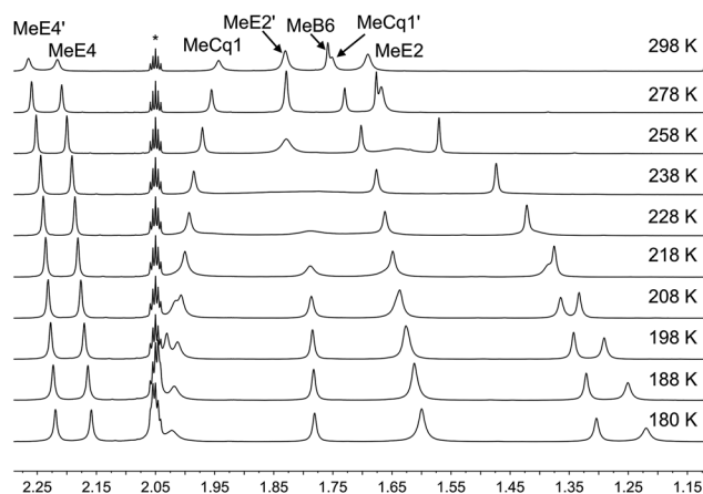
Fig. 8 Alkyl regions of the variable temperature ^1\text{H} NMR spectra (500 MHz, acetone- d_6 ) of [\text{Cu}(\text{xantphosMes}_2)(6\text{-Mebpy})][\text{PF}_6] . See Scheme 3 for atom labelling.
