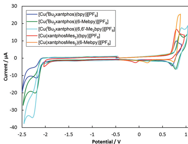
Fig. 9 Cyclic voltammograms of [\text{Cu}(\text{P}^{\wedge}\text{P})(\text{N}^{\wedge}\text{N})][\text{PF}_6] compounds in \text{CH}_2\text{Cl}_2 at a scan rate of 100 \text{ mV s}^{-1} referenced to internal \text{Fc}/\text{Fc}^+ = 0 \text{ V} .
