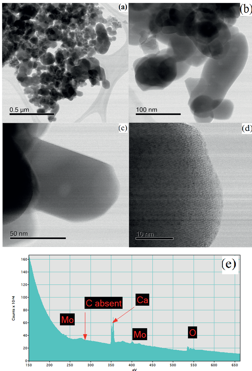
Fig. 9 STEM images of \text{CaMoO}_4 synthesized at 500 ^{\circ}\text{C} showing (a and b) a bright field image highlighting the irregular shapes and coarser particle size (50–250 nm), relative to the 300 ^{\circ}\text{C} material; (c) details of a rod-like crystal showing a single large void (bright region) approximately 10 nm in diameter; (d) an atomic resolution bright field image showing the lattice fringes to extend to the crystal edge, with no amorphous phase present; (e) EELS spectrum of (e) showing the absence of carbon.
