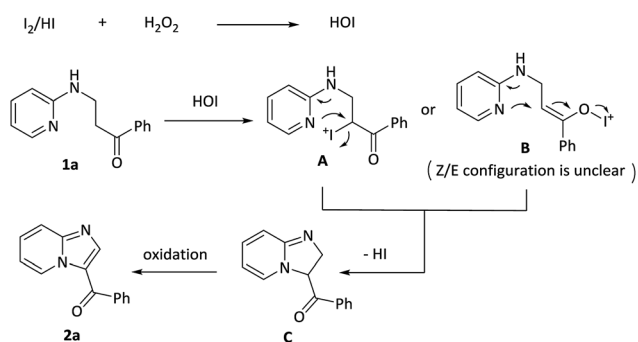
Scheme 3 Proposed mechanism.
