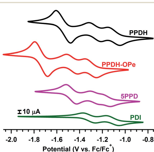
Fig. 4 Cyclic voltammograms of PPDH , PPDH-OPe , 5PPD , and monomeric PDI (1 mM, 50 mV s −1 scan rate) in Ar-sparged DCM with 0.1 M [Bu 4 N][PF 6 ] as the supporting electrolyte. For all species, R = CH(C 5 H 11 ) 2 .
