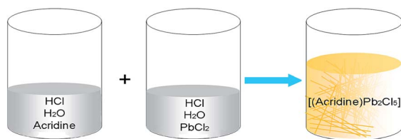
Scheme 1 The facile synthesis process of OlHP-AD perovskite crystals in aqueous solution at room temperature.
