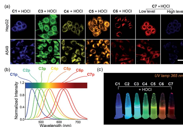
Fig. 5 (a) Confocal fluorescence images of HepG2 and A549 cells preloaded on C1 , C3–C7 (10 \mu M, 10 min) and further incubated in buffers with various concentrations of HOCl. Scale bar: 20 \mu m; (b) normalized fluorescence spectra of C1p–C7p ; (c) photographs of probes C1–C7 with the addition of HOCl were taken under illumination with a UV lamp.
