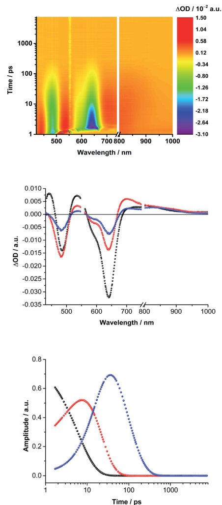
Fig. 6 (Top) Differential absorption spectra obtained by femtosecond transient absorption pump-probe experiments (550 nm, 400 nJ) of (TCBD-aniline) 3 -SubPc(TCDB-aniline) 2 ( 3 \times 10^{-5} M) in argon-saturated anisole with several time delays between 1 to 7500 ps. (Middle) Deconvoluted evolution associated spectra and (bottom) associated time-dependent amplitudes obtained via global analysis in GloTarAn monitoring formation and decay kinetics.
