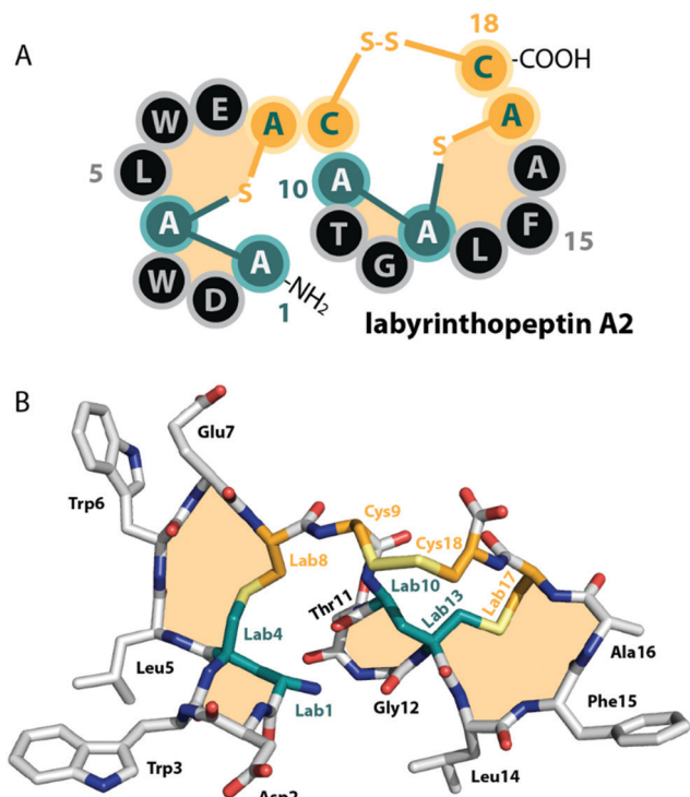
Fig. 2 (A) Schematic representation and (B) crystal structure (CCDC number 721326) of labyrinthine A2. 13 The labionin macrocycles are highlighted by orange shading in the background.
