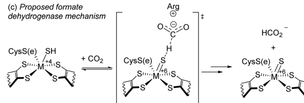
Scheme 2 (a and b) Common mechanisms for \text{CO}_2 Insertion into metal hydrides described in ref. 11, (c) proposed mechanism for hydride transfer in formate dehydrogenase described in ref. 12.
