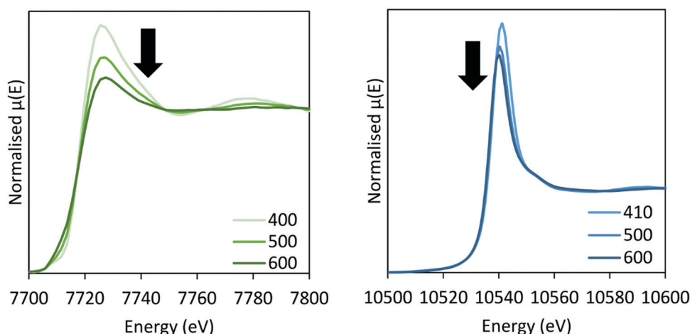
Fig. 11 XANES of the CoRe-gel during ammonia decomposition at the Co K-edge (left) and Re L_{III} -edge (right) between 400 – 600^\circ\text{C} in 5\% NH_3 .
