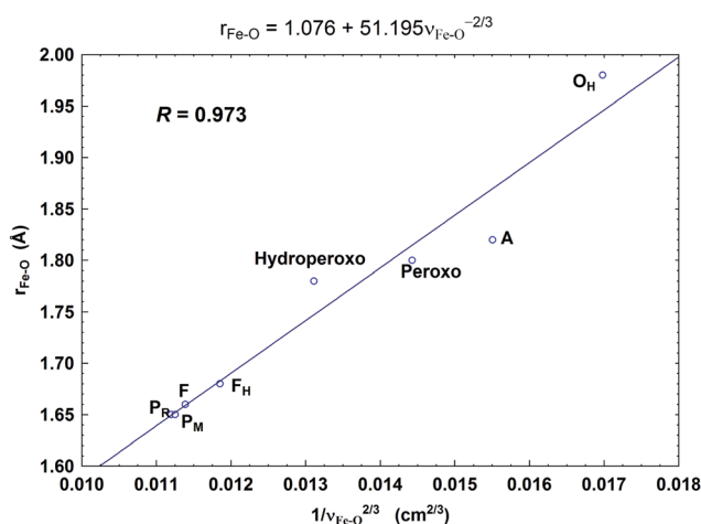
Fig. 9 Correlation between the calculated Fe a3 –O bond lengths ( r_{\text{Fe}-\text{O}} , Å) and the corresponding Fe a3 –O stretch frequencies ( 1/\nu_{\text{Fe}-\text{O}}^{2/3} , based on Badger's rule) for the eight DNC state structures studied. 59 Reprint with permission from Fig. 7 of ref. 59, copyright© 2019 American Chemical Society.
