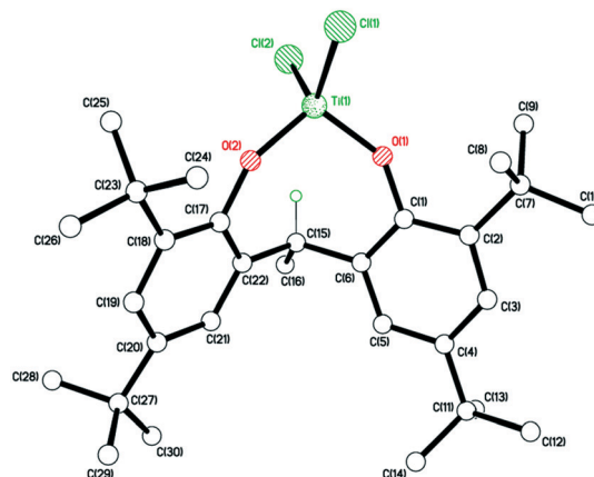
Fig. 9 Molecular structure of \{\text{TiCl}_2[2,2'-(\text{CH}_3\text{CH}[4,6-(t\text{-Bu})\text{C}_6\text{H}_2\text{O}]\text{O}_2)]\} ( 12 ) (most H atoms are omitted for clarity). Selected bond lengths (Å) and angles ( ^\circ ): Ti(1)–O(1) 1.7593(15), Ti(1)–O(2) 1.7559(14), Ti(1)–Cl(1) 2.2209(6), Ti(1)–Cl(2) 2.2284(7); C(1)–O(1)–Ti(1) 145.96(13), C(17)–O(2)–Ti(1) 151.26(13), O(2)–Ti(1)–Cl(2) 110.27(6), O(1)–Ti(1)–Cl(1) 109.15(5), O(2)–Ti(1)–O(1) 105.38(7).
