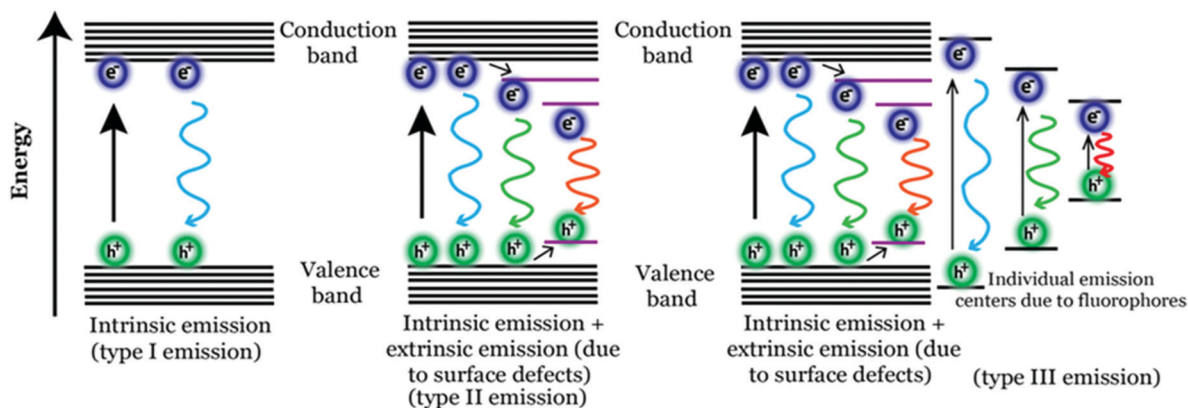
Fig. 4 Schematic representation corresponding to the emission mechanism in CdS systems.
