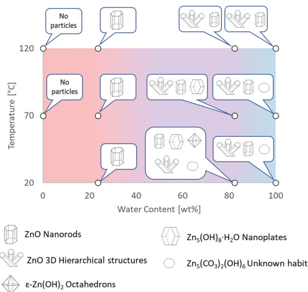
Fig. 2 Graphical summary of Zn-based materials, obtained by direct oxidation of metallic zinc in [\text{C}_4\text{C}_{1\text{im}}]\text{Cl} solutions, as a function of experimental conditions. Further details are provided in Tables S1 and S2 in ESI † .
