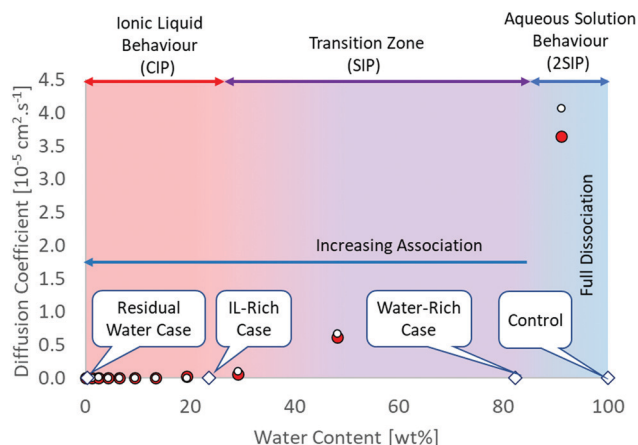
Fig. 1 Structural and diffusion properties of [\text{C}_4\text{C}_{1\text{im}}]\text{Cl}/\text{water} mixtures as a function of water concentration. Diffusion data calculated from MD simulations at 350 K. 35 White circle (○) chloride, red circle (●) [\text{C}_4\text{C}_{1\text{im}}]^+ .
