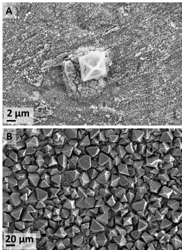
Fig. 3 SEM image showing zinc surface exposed to [\text{C}_4\text{C}_{1\text{im}}]\text{Cl} (IL-1, X_{\text{H}_2\text{O}} = 0.98 solution at 20 \pm 1 °C). (A) Single octahedron \text{Zn}(\text{OH})_2 particle after 18 d exposure (approximate length of 7.9 \pm 0.6 μm). (B) Multiple \text{Zn}(\text{OH})_2 crystals after 44 d exposure with a mean length of 21 \pm 6 μm ( n = 84 ).
