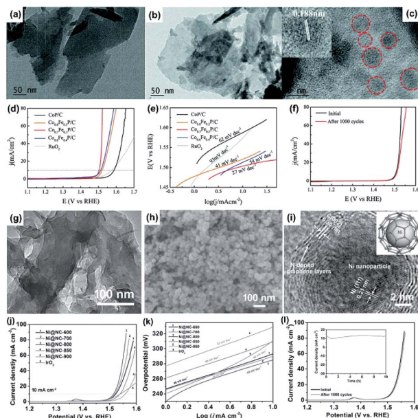
Fig. 22 TEM images of (a) \text{Co}_{0.7}\text{Fe}_{0.3}\text{-P/C} nanosheets and (b) \text{Co}_{0.7}\text{Fe}_{0.3}\text{-P/C} nanosheets. (c) HRTEM image of \text{Co}_{0.7}\text{Fe}_{0.3}\text{-P/C} nanosheets. (d) LSV curves and (e) the corresponding Tafel plots of \text{Co}_{1-x}\text{Fe}_x\text{-P/C} nanosheets and commercial \text{RuO}_2 catalyst in 1 M KOH solution. (f) Polarization curves of the \text{Co}_{0.7}\text{Fe}_{0.3}\text{-P/C} catalyst before and after 1000 potential cycles. Reproduced with permission. 197 Copyright ©2018 The Royal Society of Chemistry. (g) TEM image of Ni-BDC nanosheets. (h) SEM and (i) HRTEM images of Ni@NC. (j) The OER polarization curves and (k) the corresponding Tafel plots of various Ni@NC samples and commercial \text{IrO}_2 catalyst in 1.0 M KOH solution. (l) Polarization curves of the Ni@NC-800 catalyst before and after 1000 potential cycles. The inset of (l) is the chronoamperometric curve at 1.52 V (vs. RHE). 198 Copyright©2017 WILEY-VCH Verlag GmbH & Co. KGaA.
