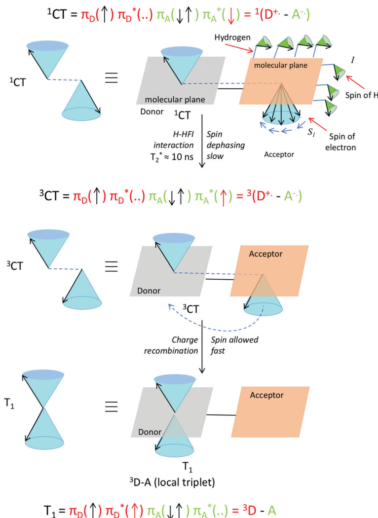
Fig. 13 Visualization of proton hyperfine interactions (H-HFI) within a co-planar electron donor–acceptor compound. Within the singlet charge-transfer excited state, the interaction between the electron spin ( S_1 ) and the nuclear spin of the H atoms ( I ), leads to slow spin dephasing ( T_2^* ). This interconverts the singlet charge-transfer excited state into the triplet charge-transfer excited state (middle). When this is formed, fast spin allowed charge recombination to a local triplet state can occur (bottom). The T_0 level is populated specifically (and not the T_+ or T_- , see also Fig. 15). The red arrow in the three electron configurations depicts the dephasing and transferring electron. A magnetic field is present in the z direction, for the purpose of simple spin representation.
