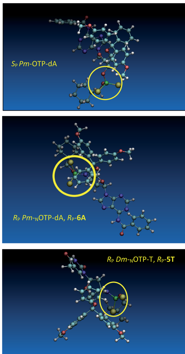
Fig. 6 Predicted by molecular modeling the lowest energy conformations of: S_P - Pm -OTP-dA, an upper panel; R_P -6A, a middle panel; R_P -5T, a bottom panel. All three compounds are P-stereochemically equivalent ( vide supra ).
