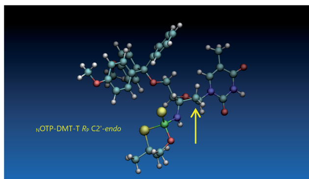
Working earlier with LNA-derived OTP monomers (OTP- \text{N}^{\text{LNA}} , which adopt the profound C3'- endo conformation), we observed (Exp. #2) that in the synthesis of per-(PS-LNA) oligonucleotides even double condensation of OTP- \text{N}^{\text{LNA}} to \text{HO}^{\text{N}^{\text{LNA}}}\text{PS} \dots \text{S} was ineffective and a \text{DMT}^+ cation absorption virtually decayed after the 5 th cycle (K. Jastrzębska, P. Guga, unpublished data); whereas, such a condensation with the 5'-OH-DNA-S proceeded with >94% efficacy. 24 As mentioned earlier, molecular modeling showed that poorly reacting 6Gf and 6Gs predominantly exist in a C3'- endo conformation. To verify whether the most reactive \text{N}^{\text{OTP-T}} monomers 5Tf and 5Ts adopt that conformation (characteristic of 3'-amino-2',3'-dideoxyribonucleosides), we performed NMR analysis.
