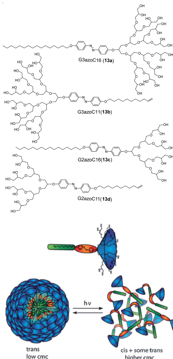
Fig. 22 Molecular structures of dendron amphiphiles ( 13a–13d ) containing azo-benzene and proposed disruption of aggregates by light through trans – cis isomerization. Reprinted from ref. 69. Copyright 2011 Royal Society of Chemistry.
