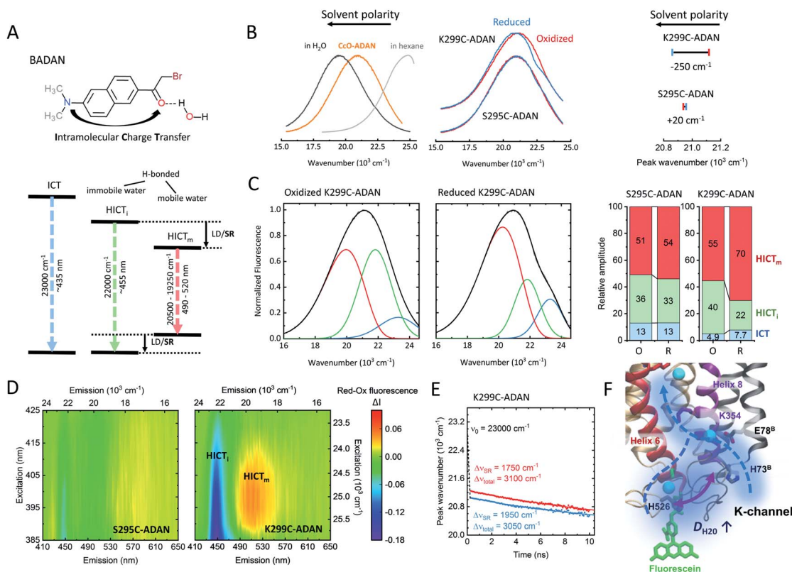
Fig. 4 (A) Chemical structure of BADAN and Jablonski diagram for the three fluorescence species (adapted from ref. 17). ICT: intramolecular charge transfer, \text{HICT}_{\text{imm}} : immobile and mobile H-bonded ICT, LD: label dynamics, SR: solvent relaxation. (B) Left: Normalized fluorescence of free BADAN in polar ( \text{H}_2\text{O} ) and nonpolar media as well as labeled to CcO. Middle: Normalized fluorescence emission spectra of oxidized (red) and reduced (blue) K299C-ADAN and S295C-ADAN. Right: Corresponding emission peak positions. Peak wavenumbers were determined through Gaussian fitting with an accuracy of 20 \text{ cm}^{-1} . (C) Spectral log-normal decomposition of oxidized and reduced K299C-ADAN. (D) Reduced-oxidized steady-state excitation-emission difference spectra of both CcO-ADAN conjugates. (E) TDFS of oxidized and reduced K299C-ADAN. (F) Scheme showing the increase in water mobility at the K-channel entrance upon CcO reduction. Experimental conditions: 20 mM potassium phosphate buffer at pH 8.0, 20 mM NaCl, 0.05% \beta -DM, 20^\circ \text{C} . Measurement accuracy: 1 nm. Experiments were performed twice.
