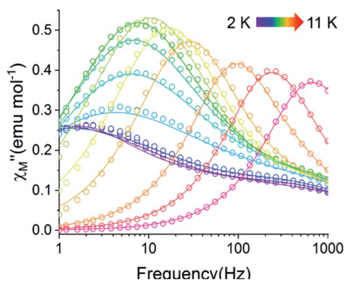
Fig. 9 Temperature dependence of the out-of-phase component of the molar ac magnetic susceptibility ( \chi''_M ) of 2 at 0.35 T ( H = 0.35 T, T = 2-11 K). Lines represent fits to the experimental data (circles).
