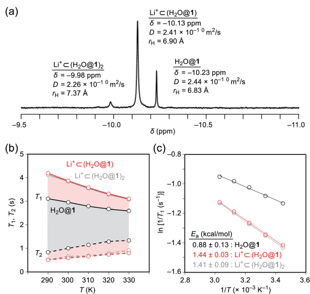
Fig. 7 (a) ^1\text{H} NMR spectrum (500 MHz, ODCB- d_4 ), (b) temperature dependence of relaxation times (errors less than 5%), and (c) Arrhenius plots ( \ln(1/T_1) vs. 1/T ) of \text{H}_2\text{O}@\mathbf{1} with 20 equiv. of \text{Li}^+[\text{B}(\text{C}_6\text{F}_5)_3]^- \cdot 2.5\text{Et}_2\text{O} (800 MHz, ODCB- d_4 ).
