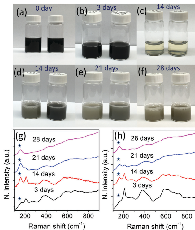
Fig. 5 Photographs of the aqueous solutions of \text{Ti}_3\text{C}_2\text{T}_x (left) and \text{r-Ti}_3\text{C}_2\text{T}_x (right) collected after (a) 0 day, (b) 3 days, (c) 14 days before shaking, (d) 14 days, (e) 21 days, and (f) 28 days. The concentrations of \text{Ti}_3\text{C}_2\text{T}_x and \text{r-Ti}_3\text{C}_2\text{T}_x solutions were 15 mg in 10 ml of water. Normalized Raman spectra collected on dried powder from the aqueous solutions of (g) \text{Ti}_3\text{C}_2\text{T}_x , and (h) \text{r-Ti}_3\text{C}_2\text{T}_x kept for different days.
