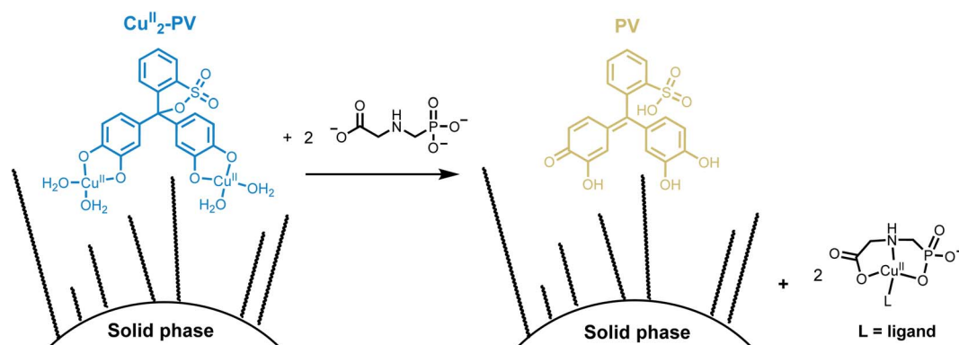
Fig. 2 Schematic representation of detection of GlyP with an immobilized \text{Cu}^{II} -PV complex by an indicator displacement assay using solid phase extraction.
