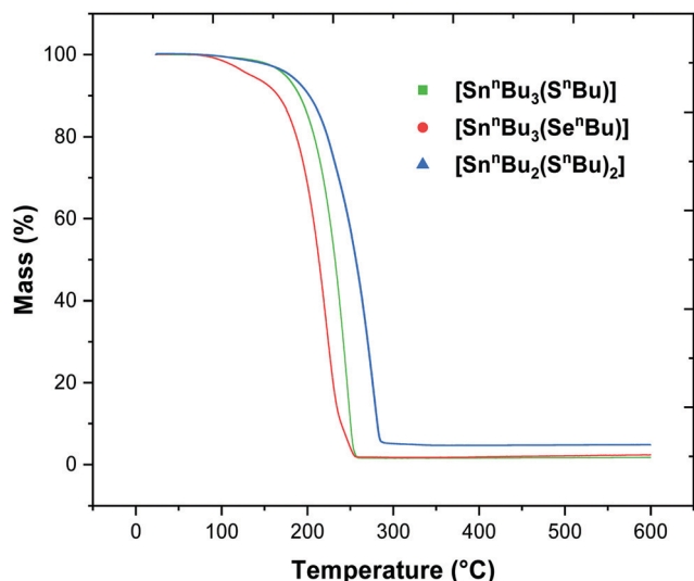
Fig. 1 TGA profiles for (1) (green), (2) (blue) and (3) (red). The TGA experiments were conducted with a temperature ramp rate of 5 °C min -1 and a constant flow of argon gas at a flow rate of 30 mL min -1 .
