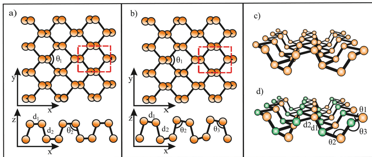
Fig. 18 (a) Scheme of the symmetric puckered or washboard structure sw-X . The red dashed lines label the rectangular unit cell with four atoms. (b) Scheme of the asymmetric puckered or washboard structure aw-X . The red dashed lines label the rectangular unit cell with four atoms. (c) Perspective view of the asymmetric puckered structure aw-X . (d) Perspective view of the asymmetric puckered structure of binary group V monolayers.
