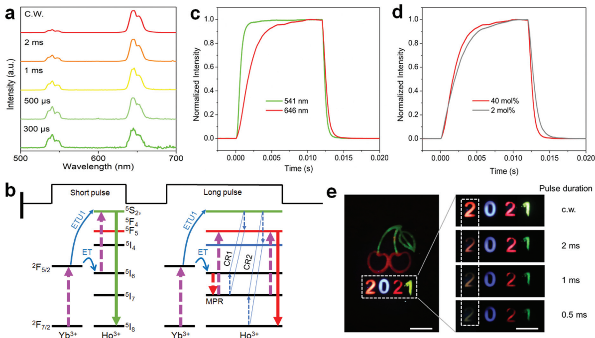
Fig. 7 (a) Upconversion emission spectra of \text{NaYF}_4:\text{Ho}(40\text{ mol}\%)@ \text{NaYF}_4:\text{Yb}(60\text{ mol}\%)@ \text{NaYF}_4 core–shell–shell nanoparticles under pulsed 980 nm excitation with a tuning of the pulse duration. (b) Schematic of the possible processes for the reduction of the red upconversion under non-steady state excitation. (c) Time-dependent emission profiles of \text{Ho}^{3+} at 541 and 646 nm of (a) sample under 980 nm irradiation with a pulse duration of 12 ms (50 Hz). (d) A comparison of the time-dependent red upconversion emission profiles from the (a) sample and \text{NaYF}_4:\text{Yb}/\text{Ho}(20/2\text{ mol}\%)@ \text{NaYF}_4 core–shell nanoparticles. (e) Schematic of decoding the concealed information on the cherry pattern under pulsed 980 nm irradiation (right panels) in which only the initial number “2” shows a color change with reducing the pulse duration. Scale bars, 0.5 cm.
